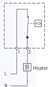
Wiring Diagram
