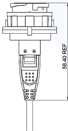
Dimensions figure
