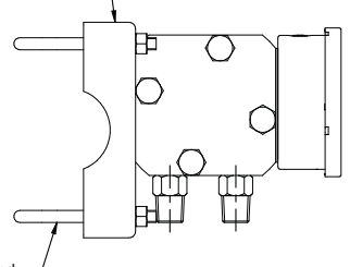
2" Pipe Mounting Bracket.
