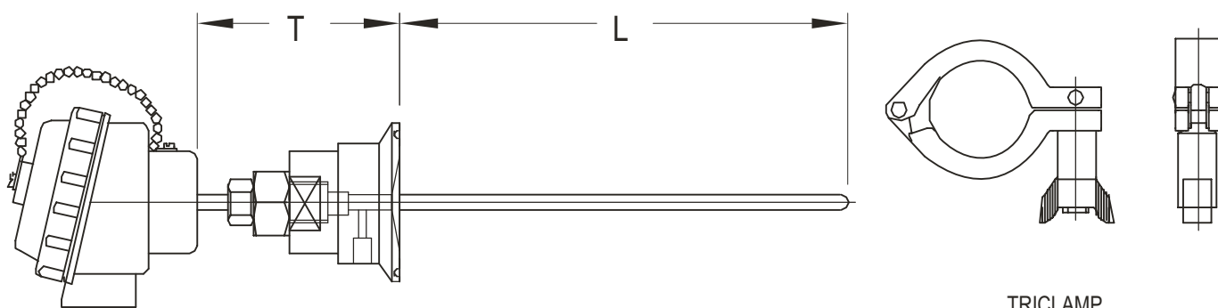
TRICLAMP
